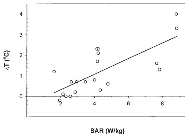
Fig. 3. Dependence of temperature rise, relative to the unexposed control, on specific absorption rate (SAR) levels.
